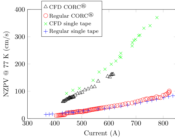
Figure 12. NZPV obtained at 77 K in self-field versus applied current for the CFD CORC® cable (black triangles), and the regular CORC® cable (red circles). The NZPV of a CFD tape (green (x)) and a regular tape (blue +) divided by the length ratio p are also shown. For comparison, the applied current applied on the single tapes was multiplied by a factor of six, i.e. the number of tapes in the CORC® cables.
