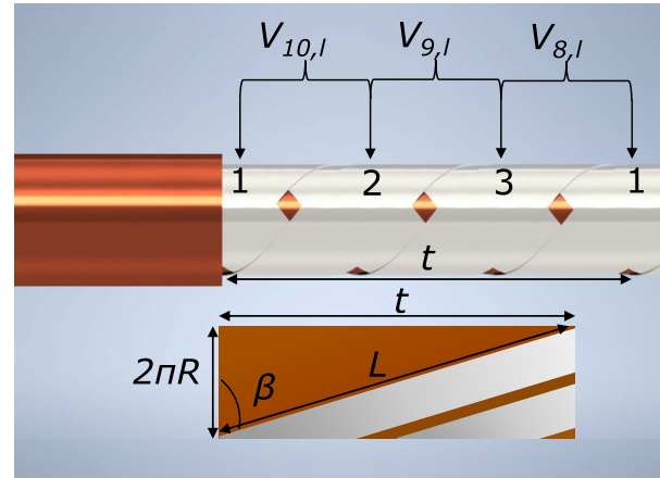
Figure 4. Top figure: schematic of the position of the voltage taps ( V_{i,l} , i = 10, 9, 8, l = \text{left} ) on the outer layer of the CORC® cable. Bottom figure: schematic of REBCO tapes in a CORC® cable in a rectangular plane showing the length L of a straight piece of REBCO tape along a full twist pitch t , and the twist angle of the outer layer \beta .
